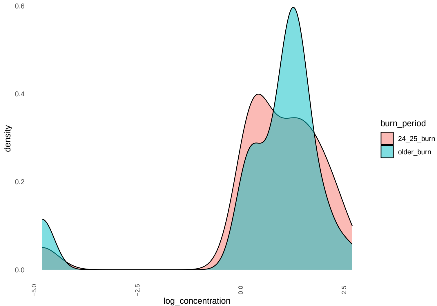
DOC log-concentration: shrub_grass by burn period
